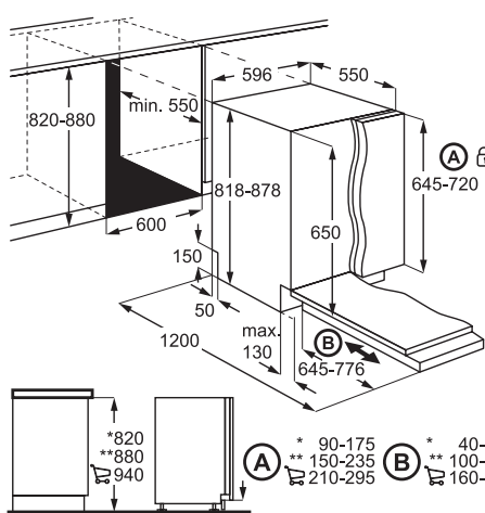
FSK52917Z, FSK52617Z, FSB42607Z FULLY INTEGRATED
