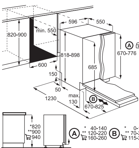
FSK93807P, FSK84707P, FSK63807P, FSK63730P, FSK62607P FULLY INTEGRATED
