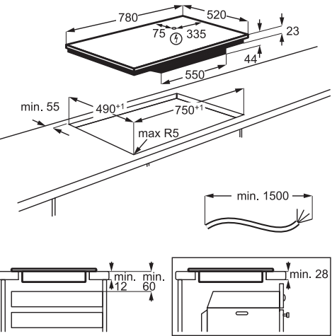
IKE84471FB, IKE85431FB, IAE84411FB, IKE84441FB, IKB84401FB
