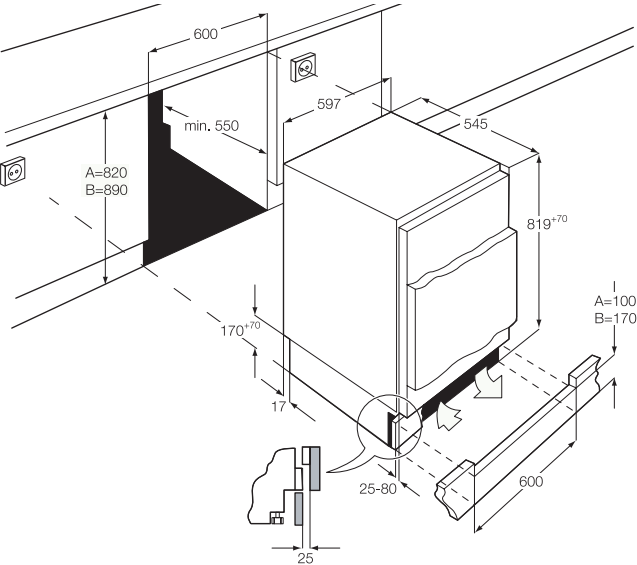
ABE6821VNF, ABE6822VAF, ABB6821VAF, SFE5822VAF, SFB5821VAF, SKE5822VAF, SKB5821VAF
