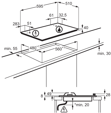
HG654550SY, HG654351SM, HG644351SM
