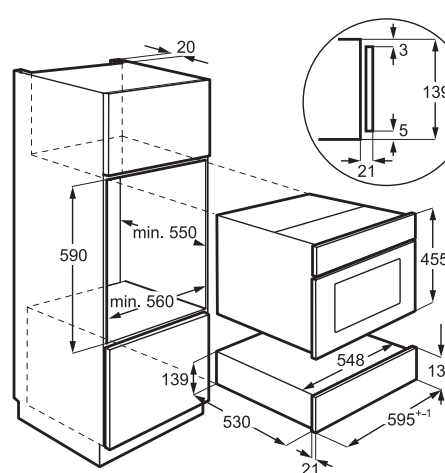
KDK911424M, KDE911424M, KDE911424B
